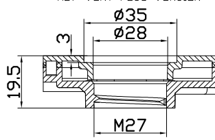
PUSH IN VENT PLUG VERSION
