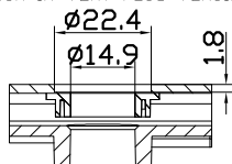
PUSH IN VENT PLUG VERSION
