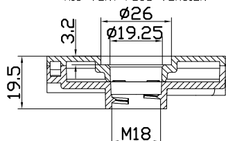
PUSH IN VENT PLUG VERSION
