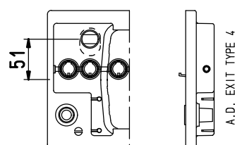
PEEPHOLE Ø20.4 IMBL VERSION
