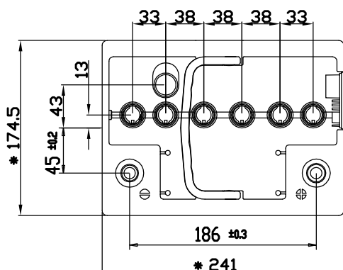
PEEPHOLE Ø20.4 VERSION
